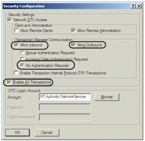
Figure 7-25: Security Configuration Window
