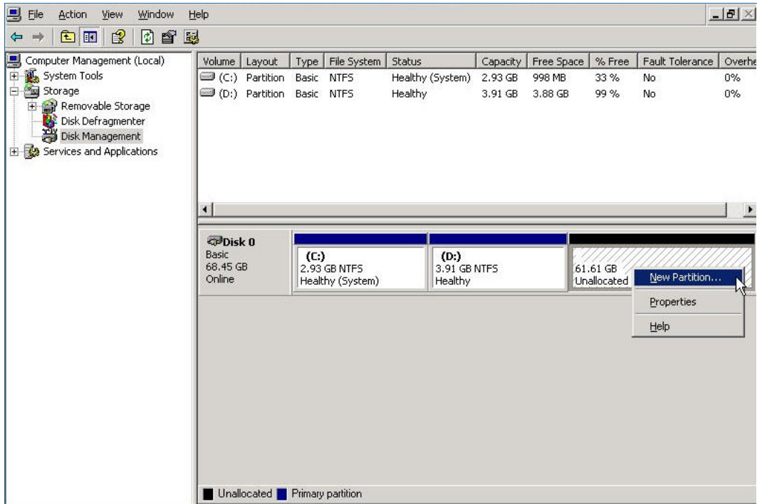
Figure 3-32: Disk Management
